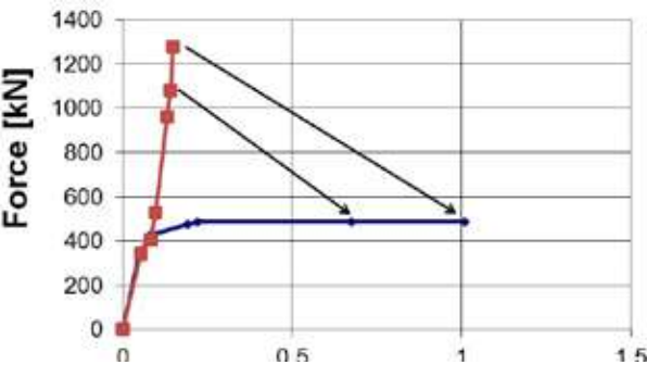
Fig. 8. Result of the pushover (blue curve) on an equivalent structure leading to an estimation of function in Risk’s General Equations (red curve).
