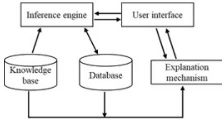
Fig. 3. Expert system structure.
