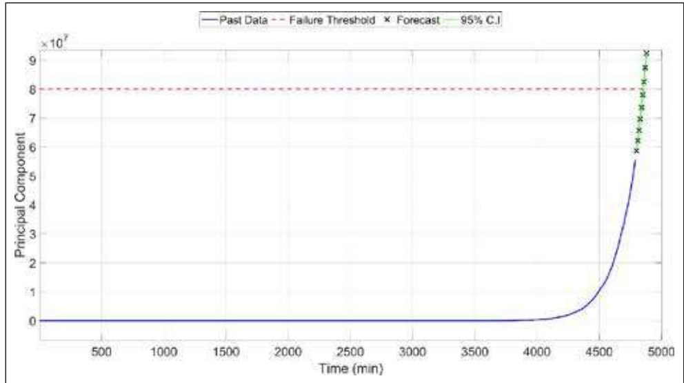
Fig. 5. Estimated values of the first principal component using the degradation model
