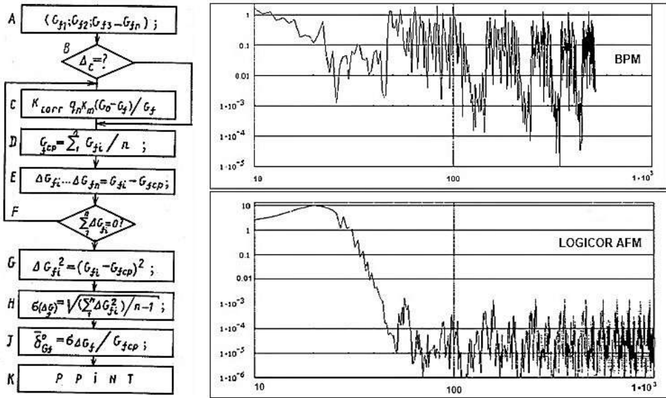
Fig 6. The results of tests BPM and Logikor-AFM classification and correction algorithms for the IoT-CPS platform
