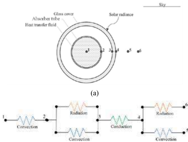
Fig.1. Receiver tube: a) cross sectional view and b) thermal resistance model
