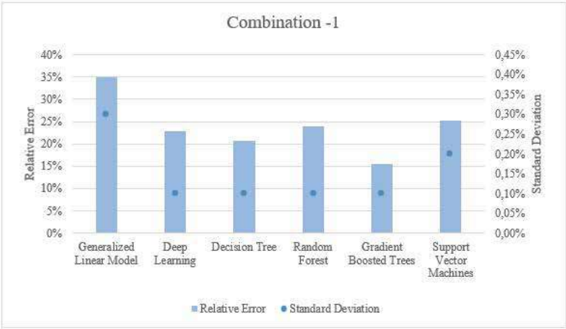
Fig. 1. RapidMiner Studio Output - Model 1
