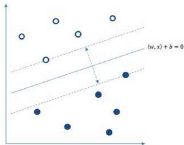
Fig. 4. Support Vector Machine Method [3].
