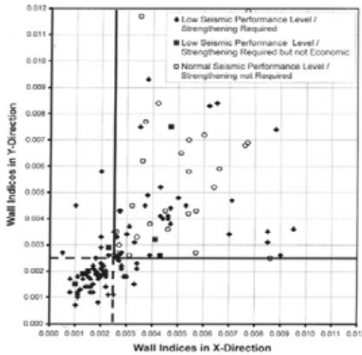
Fig. 8. Wall indices for seismic performance evaluation database.
