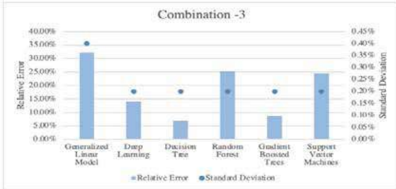
Fig. 3: RapidMiner Studio Output - Model 3
