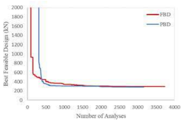
Fig. 4. Optimization histories for PBD and FBD of 54-member planar OMRSF
